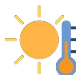
Diagram 2. Climate change projections for the Cayman Islands.
