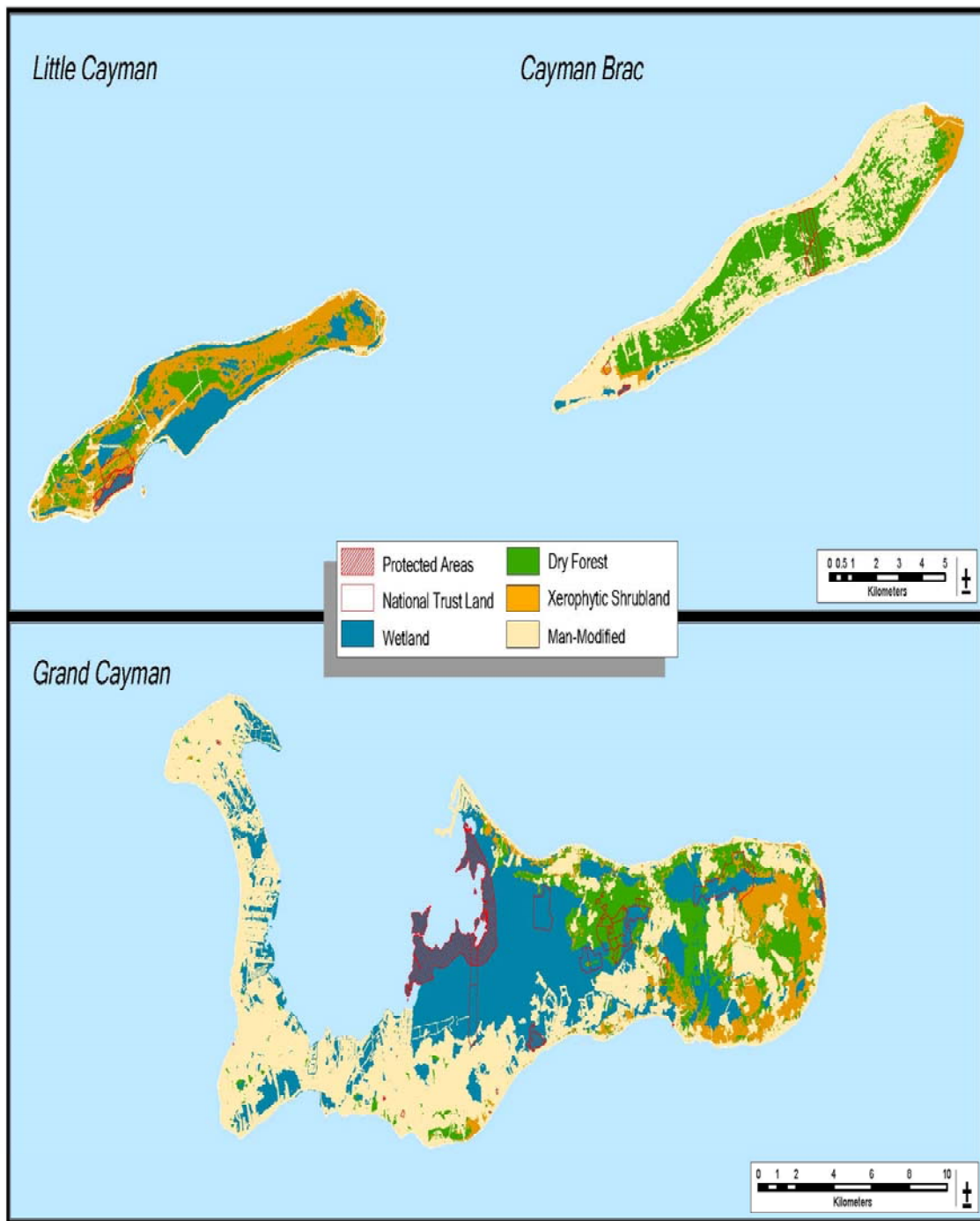
Chart 5.05: Cayman Islands Landcover Classification, 2006
